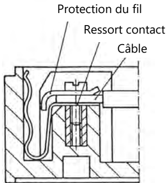
Figure 1 : Câblage
