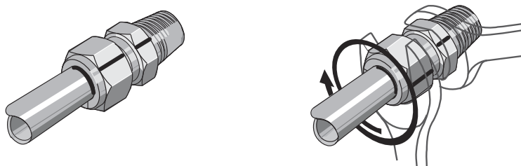
Figure4: Tightening the compression fitting
